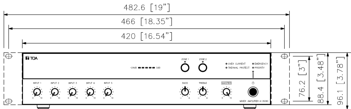
Front View
